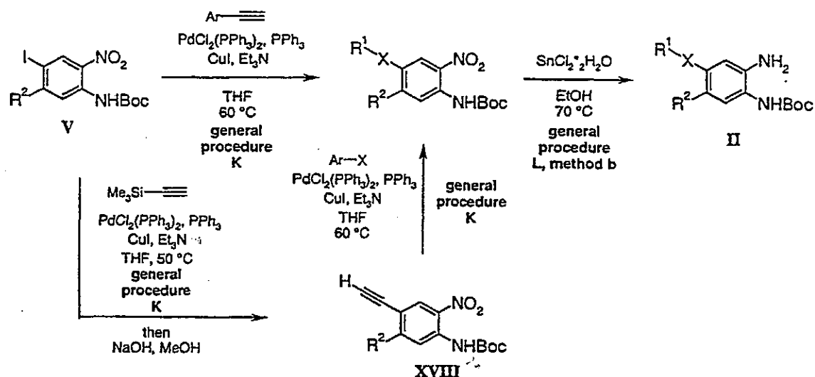
Scheme G
