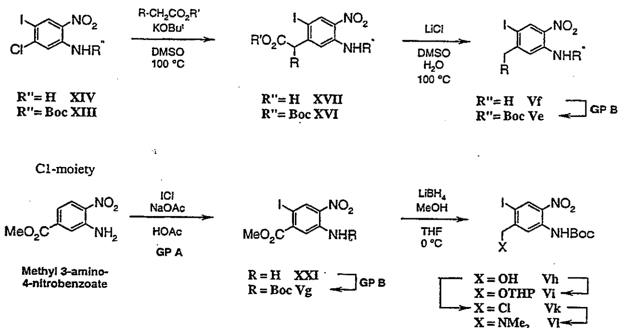
Carbon nucleophiles
