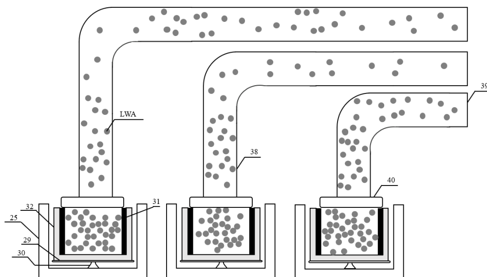
Figure 6: Sectional view of the unloading device of the furnace chamber
