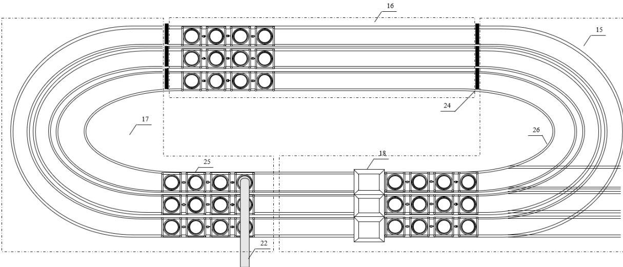
Figure 2: Configuration of the furnace chamber
