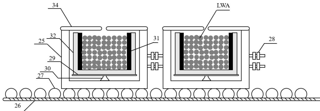
Figure 3: Sectional view of transmission device of the furnace chamber
