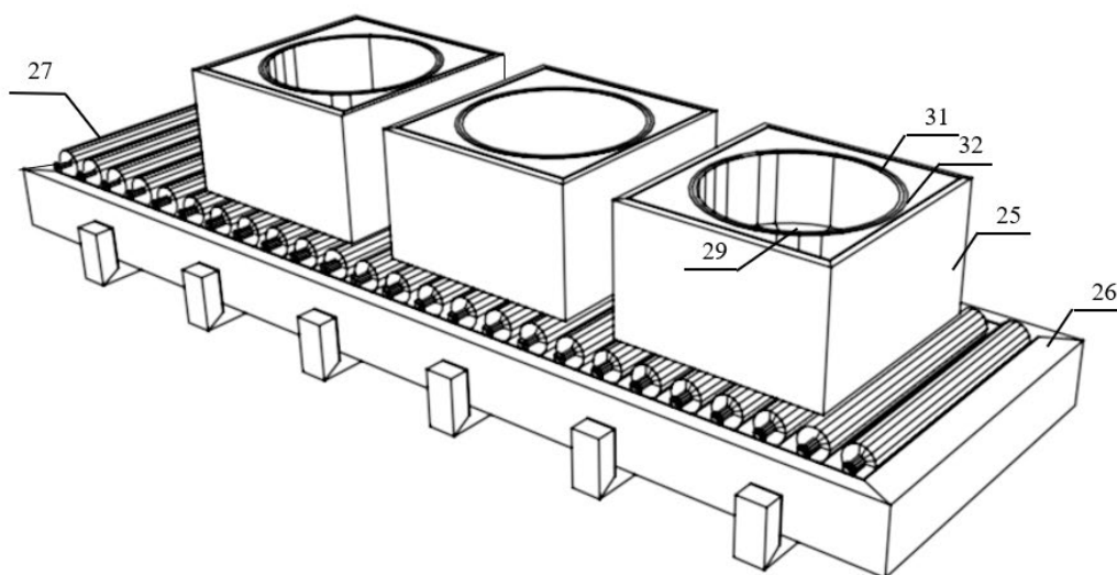
Figure 5: Perspective view of the transmission device of the furnace chamber
