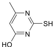
2-mercapto-6-methylpyrimidin-4-ol
