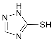
1 H -1,2,4-triazole-5-thiol
