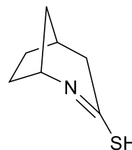
2-azabicyclo[3.2.1]oct-2-ene-3-thiol (VIVg)
