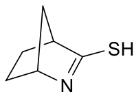
2-azabicyclo[2.2.1]hept-2-ene-3-thiol (VIVf)
