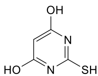
2-mercaptopyrimidine-4,6-diol
