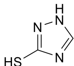
1 H -1,2,4-triazole-3-thiol (VIV)
