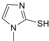
1-methyl-1 H -imidazole-2-thiol (VIVn)
