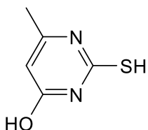
2-mercapto-6-methylpyrimidin-4-ol
