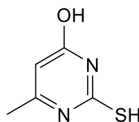
2-mercapto-6-methylpyrimidin-4-ol (VIVi)
