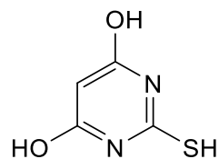
2-mercaptopyrimidine-4,6-diol
