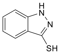
1 H -indazole-3-thiol (VIVp)
