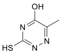
3-mercapto-6-methyl-1,2,4-triazin-5-ol
