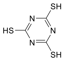
1,3,5-triazine-2,4,6-trithiol (VIVh)
