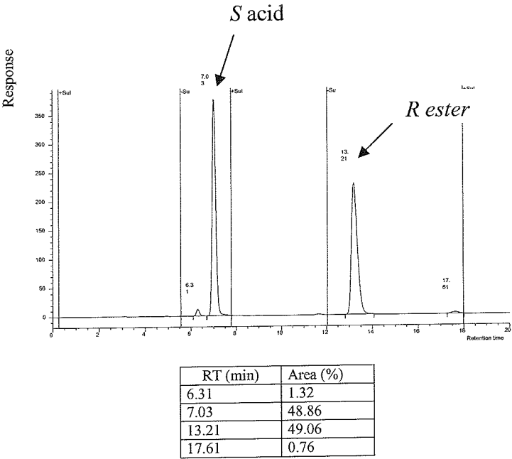
Figure 2 – Enzymatic esterification after 48 hrs.
