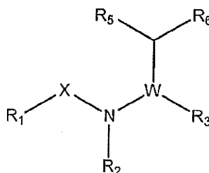
(Formula XIII)
