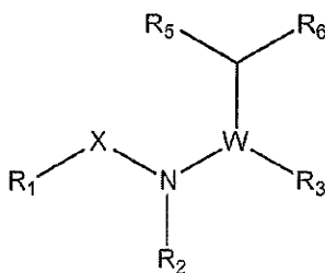
(Formula VIII)
