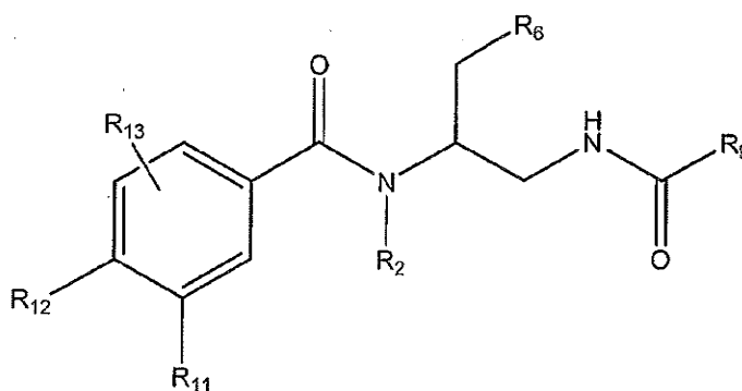
(Formula VII)
