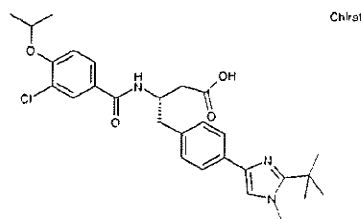
(3S)-3-[(3-Chloro-4-[(1-methylethyl)oxy]phenyl)carbonyl]amino-4-{4-[2-(1,1-dimethylethyl)-1-methyl-1H-imidazol-4-yl]phenyl}butanoic acid
