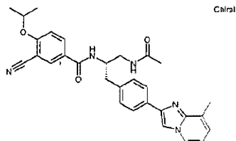
N-((1S)-2-(Acetylamino)-1-{{4-(8-methylimidazo[1,2-a]pyridin-2-yl)phenyl]methyl}ethyl)-3-cyano-4-[(1-methylethyl)oxy]benzamide
