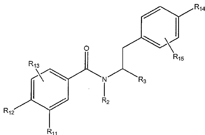
(Formula V)
