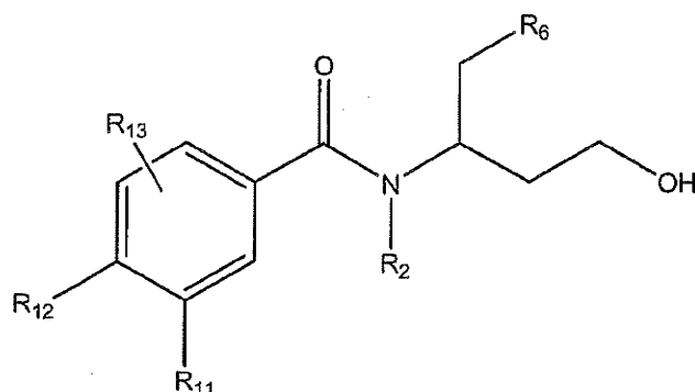
(Formula IV)
