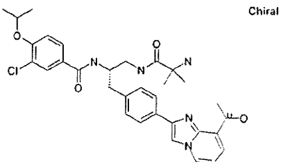
3-Chloro- N -((1 S )-2-{4-[8-(1-hydroxyethyl)imidazo[1,2- a ]pyridin-2-yl]phenyl}-1-[(2-methylalanyl)amino]methyl)ethyl)-4-[(1-methylethyl)oxy]benzamide
