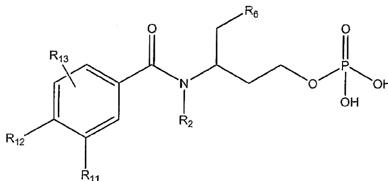
(Formula VI)
