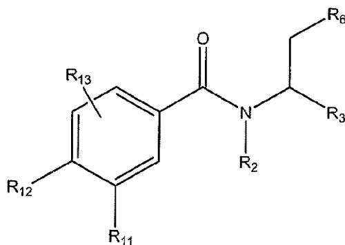
(Formula III)
