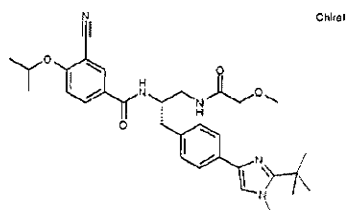
N-[(S)-1-[4-(2-tert-Butyl-1-methyl-1H-imidazol-4-yl)-benzyl]-2-(2-methoxy-ethanoylamino)-ethyl]-3-cyano-4-isopropoxy-benzamide
