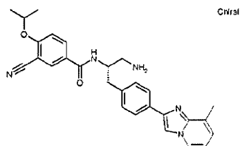
N-((1S)-2-Amino-1-{{4-(8-methylimidazo[1,2-a]pyridin-2-yl)phenyl]methyl}ethyl)-3-cyano-4-[(1-methylethyl)oxy]benzamide
