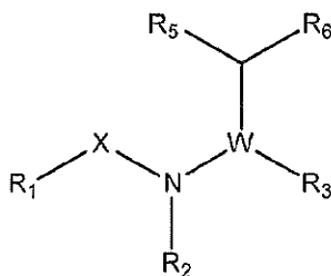
(Formula XI)
