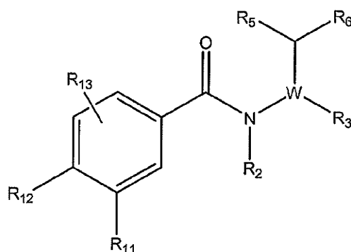
(Formula II)
