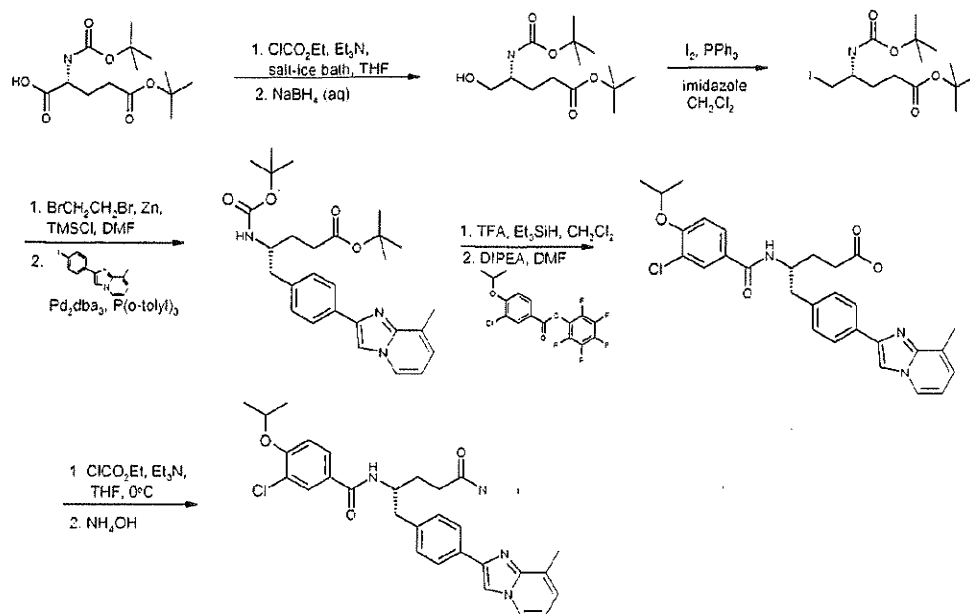
Scheme H:
