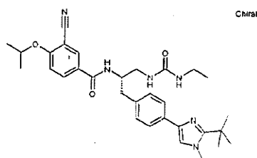
3-Cyano-N-[(1S)-2-{4-[2-(1,1-dimethylethyl)-1-methyl-1H-imidazol-4-yl]phenyl}-1-({[(ethylamino)carbonyl]amino}methyl)ethyl]-4-[(1-methylethyl)oxy]benzamide
