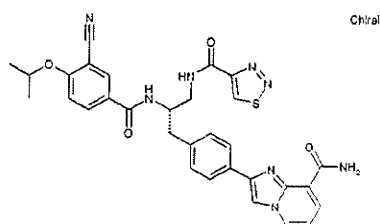
2-(4-{(2S)-2-[(3-Cyano-4-[(1-methylethyl)oxy]phenyl)carbonyl]amino}-3-[(1,2,3-thiadiazol-4-ylcarbonyl)amino]propyl}phenyl)imidazo[1,2-a]pyridine-8-carboxamide
