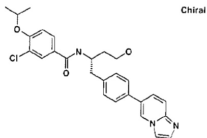
3-Chloro- N -{(1 S )-3-hydroxy-1-[(4-imidazo[1,2- a ]pyridin-6-yl)phenyl]methyl}propyl}-4-[(1-methylethyl)oxy]benzamide
