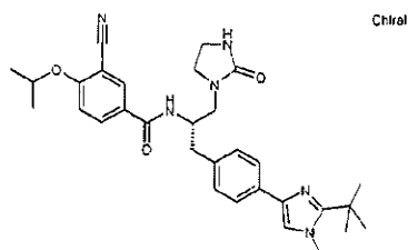
3-Cyano-N-((1S)-2-{{4-[2-(1,1-dimethylethyl)-1-methyl-1H-imidazol-4-yl]phenyl}-1-[(2-oxo-1-imidazolidinyl)methyl]ethyl}-4-[(1-methylethyl)oxy]benzamide
