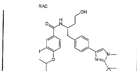
(S)-3-chloro-N-(1-(4-(1-ethyl-2-(2-hydroxypropan-2-yl)-1H-imidazol-4-yl)phenyl)-4-hydroxybutan-2-yl)-4-isopropoxybenzamide
