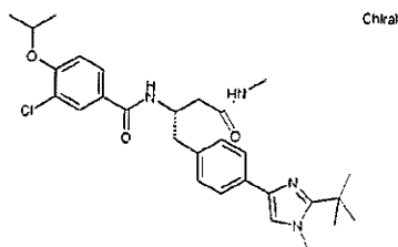
3-Chloro-N-[(1S)-1-({4-[2-(1,1-dimethylethyl)-1-methyl-1H-imidazol-4-yl]phenyl}methyl)-3-(methylamino)-3-oxopropyl]-4-[(1-methylethyl)oxy]benzamide
