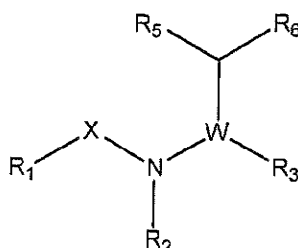
(Formula XII)
