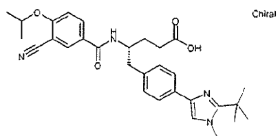
(4R)-4-[[[3-Cyano-4-[(1-methylethyl)oxy]phenyl]carbonyl]amino]-5-{4-[2-(1,1-dimethylethyl)-1-methyl-1H-imidazol-4-yl]phenyl}pentanoic acid
