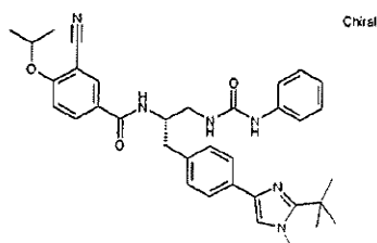
3-Cyano-N-[(1S)-2-{4-[2-(1,1-dimethylethyl)-1-methyl-1H-imidazol-4-yl]phenyl}-1-({[(phenylamino)carbonyl]amino}methyl)ethyl]-4-[(1-methylethyl)oxy]benzamide
