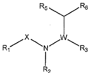
(Formula X)
