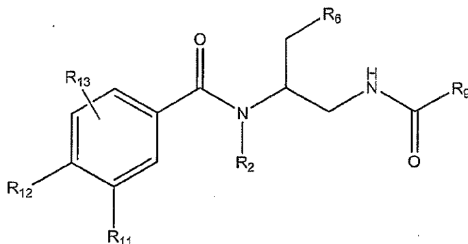
(Formula VII)
