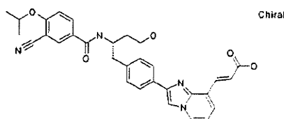
(2 E )-3-[2-(4-[(2 S )-2-[(3-Cyano-4-[(1-methylethyl)oxy]phenyl)carbonyl]amino]-4-hydroxybutyl)phenyl]imidazo[1,2- a ]pyridin-8-yl]-2-propenoic acid
