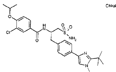
N-[(1S)-2-(Aminosulfonyl)-1-({4-[2-(1,1-dimethylethyl)-1-methyl-1H-imidazol-4-yl]phenyl}methyl)ethyl]-3-chloro-4-[(1-methylethyl)oxy]benzamide
