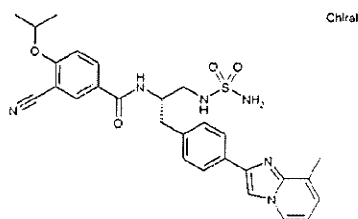
N-((1S)-2-[(Aminosulfonyl)amino]-1-{[4-(8-methylimidazo[1,2-a]pyridin-2-yl)phenyl]methyl}ethyl)-3-cyano-4-[(1-methylethyl)oxy]benzamide
