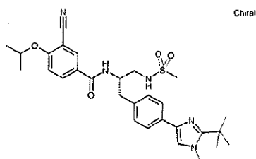
3-Cyano-N-((1S)-2-{4-[2-(1,1-dimethylethyl)-1-methyl-1H-imidazol-4-yl]phenyl}-1-[[methylsulfonyl]amino]methyl]ethyl)-4-[(1-methylethyl)oxy]benzamide
