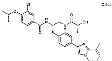
3-Chloro-N-((1S)-2-{{[(2R)-2-hydroxypropanoyl]amino}-1-{{4-(8-methylimidazo[1,2-a]pyridin-2-yl)phenyl]methyl}ethyl}-4-[(1-methylethyl)oxy]benzamide
