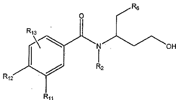
(Formula IV)
