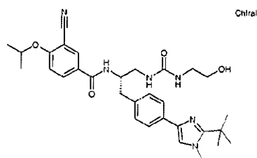
3-Cyano-N-((1S)-2-{4-[2-(1,1-dimethylethyl)-1-methyl-1H-imidazol-4-yl]phenyl}-1-[[[(2-hydroxyethyl)amino]carbonyl]amino]methyl]ethyl)-4-[(1-methylethyl)oxy]benzamide
