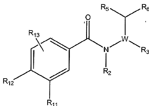
(Formula II)
