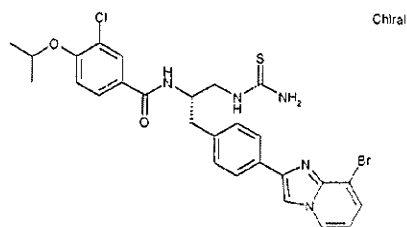
N-((1S)-2-[(Aminocarbonothioyl)amino]-1-{[4-(8-bromoimidazo[1,2-a]pyridin-2-yl)phenyl]methyl}ethyl)-3-chloro-4-[(1-methylethyl)oxy]benzamide
