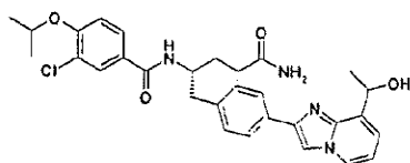
N -[(1 R )-4-Amino-1-({4-[8-(1-hydroxyethyl)imidazo[1,2- a ]pyridin-2-yl]phenyl)methyl}-4-oxobutyl]-3-chloro-4-[(1-methylethyl)oxy]benzamide
