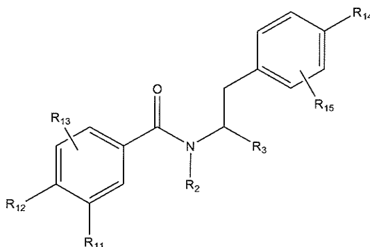
(Formula V)
