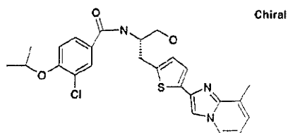
3-Chloro- N -[(1 S )-2-hydroxy-1-([5-(8-methylimidazo[1,2- a ]pyridin-2-yl)-2-thienyl]methyl)ethyl]-4-[(1-methylethyl)oxy]benzamide
