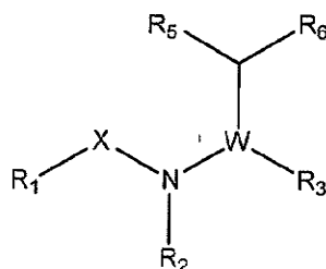
(Formula IX)
