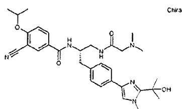
3-Cyano-N-[(1S)-2-[(N,N-dimethylglycyl)amino]-1-({4-[2-(1-hydroxy-1-methylethyl)-1-methyl-1H-imidazol-4-yl]phenyl} methyl)ethyl]-4-[(1-methylethyl)oxy]benzamide
