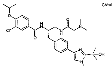
3-Chloro-N-[(1S)-2-[(N,N-dimethylglycyl)amino]-1-({4-[2-(1-hydroxy-1-methylethyl)-1-methyl-1H-imidazol-4-yl]phenyl} methyl)ethyl]-4-[(1-methylethyl)oxy]benzamide
