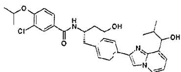
3-Chloro- N -[(1 S )-3-hydroxy-1-({4-[8-(1-hydroxy-2-methylpropyl)imidazo[1,2- a ]pyridin-2-yl]phenyl)methyl}propyl)-4-[(1-methylethyl)oxy]benzamide
