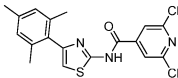
2,6-Dichloro-N-(4-mesitylthiazol-2-yl)isonicotinamide compound 88
