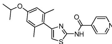
N-(4-(4-Isopropoxy-2,6-dimethylphenyl)thiazol-2-yl)isonicotinamide compound 82
