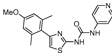
1-(4-(4-Methoxy-2,6-dimethylphenyl)thiazol-2-yl)-3-(pyridin-4-yl)urea compound 67
