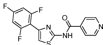
N-(4-(2,4,6-Trifluorophenyl)thiazol-2-yl)isonicotinamide compound 76
