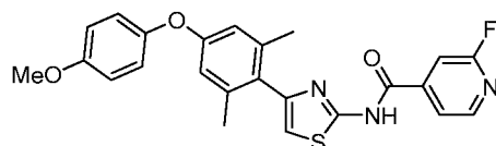
2-Fluoro-N-(4-(4-(4-methoxyphenoxy)-2,6-dimethylphenyl)thiazol-2-yl)isonicotinamide compound 98
