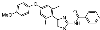
N-(4-(4-(4-Methoxyphenoxy)-2,6-dimethylphenyl)thiazol-2-yl)isonicotinamide compound 95
