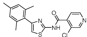
3-Chloro-N-(4-mesitylthiazol-2-yl)isonicotinamide compound 80
