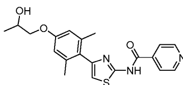
N-(4-(4-(2-Hydroxypropoxy)-2,6-dimethylphenyl)thiazol-2-yl)isonicotinamide compound 94
