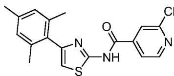
2-Chloro-N-(4-mesitylthiazol-2-yl)isonicotinamide compound 81
