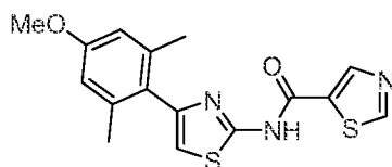
N-(4-(4-Methoxy-2,6-dimethylphenyl)thiazol-2-yl)thiazole-5-carboxamide compound 75
