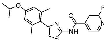
2-Fluoro-N-(4-(4-isopropoxy-2,6-dimethylphenyl)thiazol-2-yl)isonicotinamide compound 99
