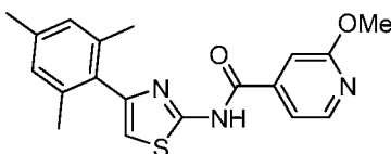
N-(4-Mesitylthiazol-2-yl)-2-methoxyisonicotinamide compound 86
