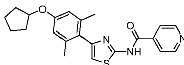
N-(4-(4-(Cyclopentyloxy)-2,6-dimethylphenyl)thiazol-2-yl)isonicotinamide compound 85
