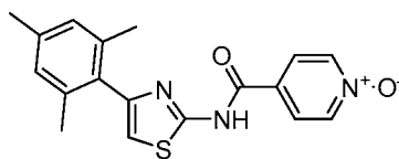
4-(4-Mesitylthiazol-2-ylcarbamoyl)pyridine 1-oxide
