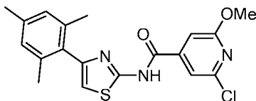
2-Chloro-N-(4-mesitylthiazol-2-yl)-6-methoxyisonicotinamide compound 87
