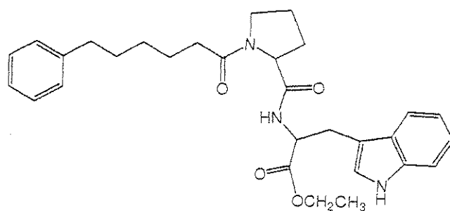
Compound V
