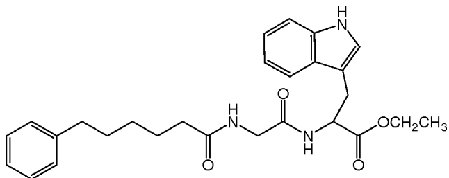
Compound S
