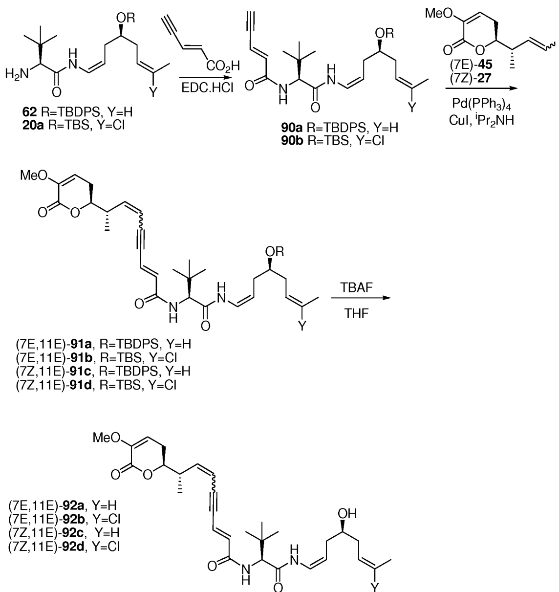
Scheme 19
