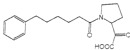
Compound Z.
