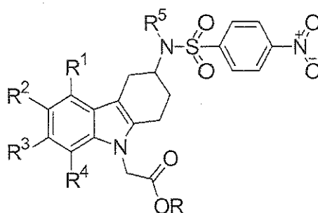
Structure 3a , wherein R^5 represents H
