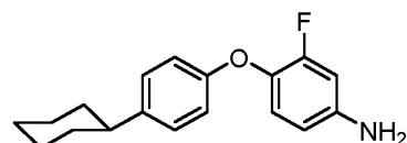
4-(4-Cyclohexylphenoxy)-3-fluoroaniline,
