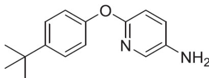
Formula (Ia)
