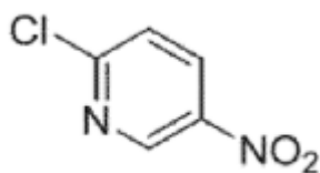
Formula (IVa)
