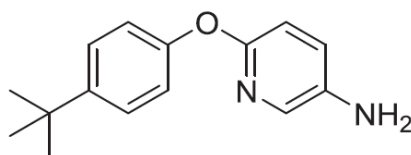
Formula (Ia)
