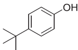
Formula (IIIa)
