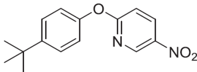
Formula (IIa)
