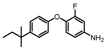
3-Fluoro-4-(4-(tert-pentyl)phenoxy)aniline,
