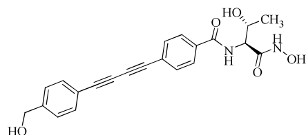
Compound C
