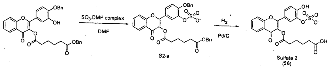
Figure 5: Synthesis of sulfate 2 (56)
