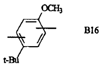
[Chemical Formula 8]
