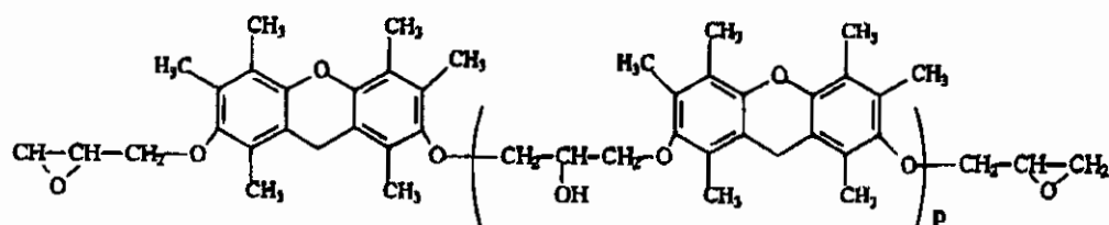
[Chemical Formula 19]
