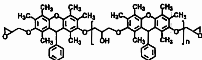
[Chemical Formula 34]
