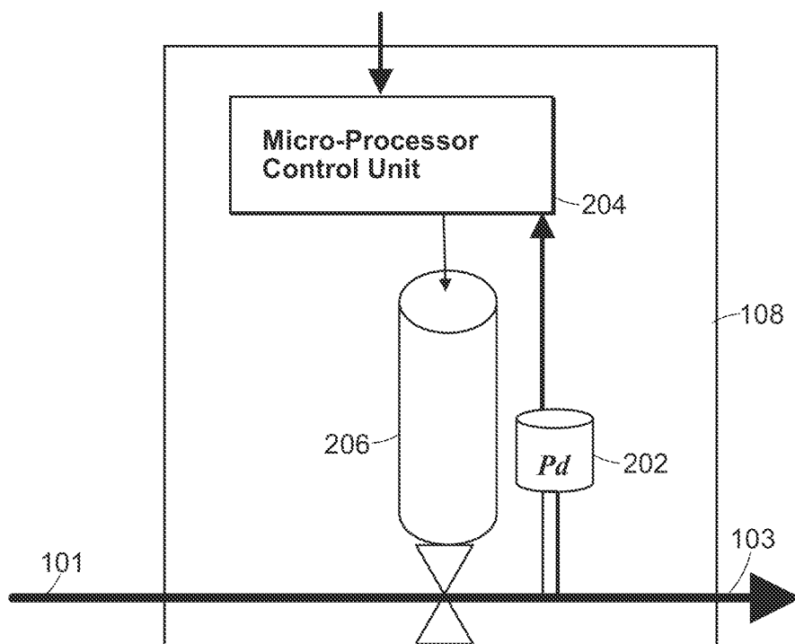
FIG. 2 (Prior Art)
