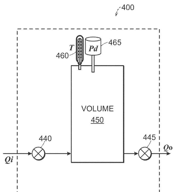
FIG. 4 (Prior Art)
