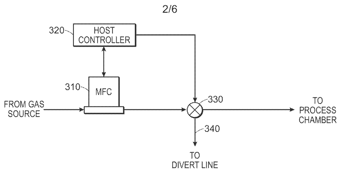
FIG. 3 (Prior Art)
