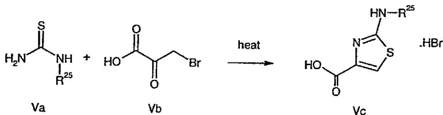
Scheme V
