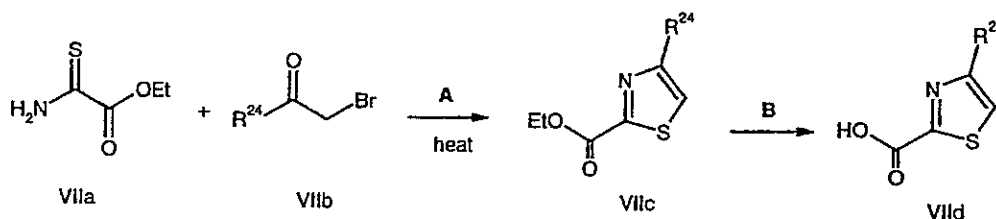
Scheme VII
