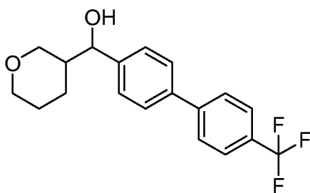
diastereomer A
