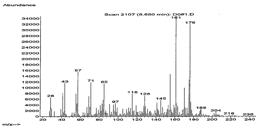
Figure 3. MS spectrum of trimethyl BTH.
