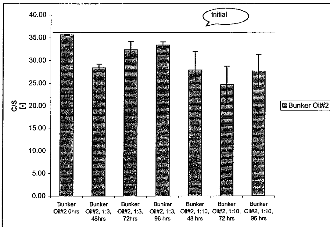
Figure 25c. C/S ratio for Bunker Oil #2 using Elemental Analyzer.
