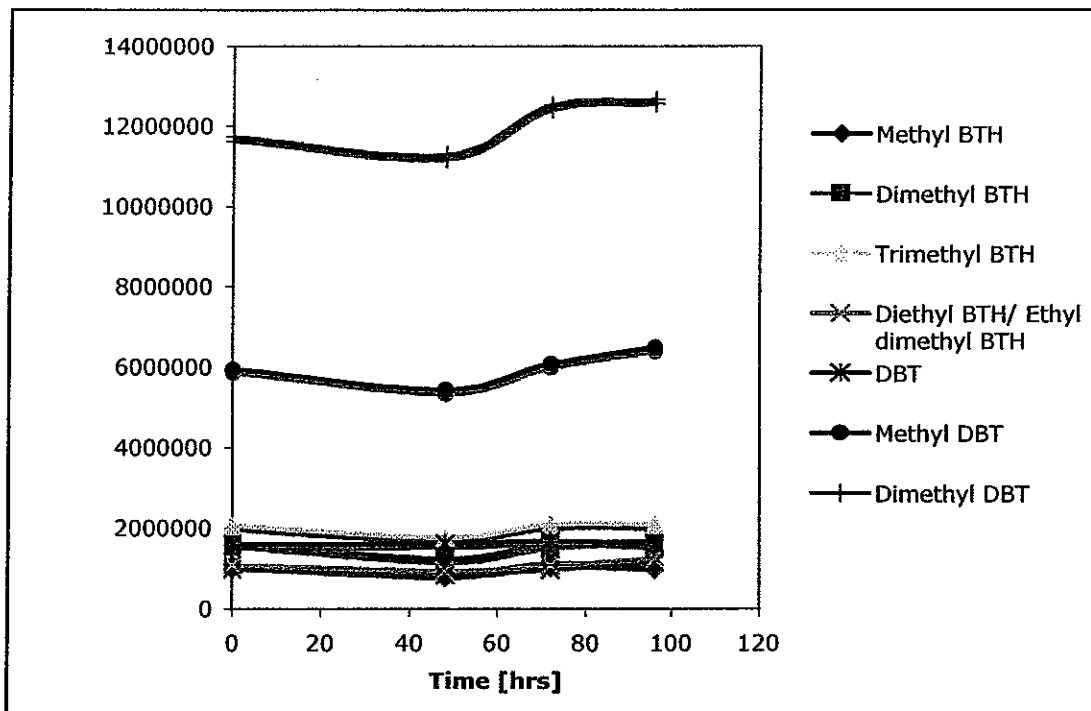
Figure 22. Change in intensity of organosulfur species over time course for Bunker Oil #2 (Vol. Oil/Water 1:3).
