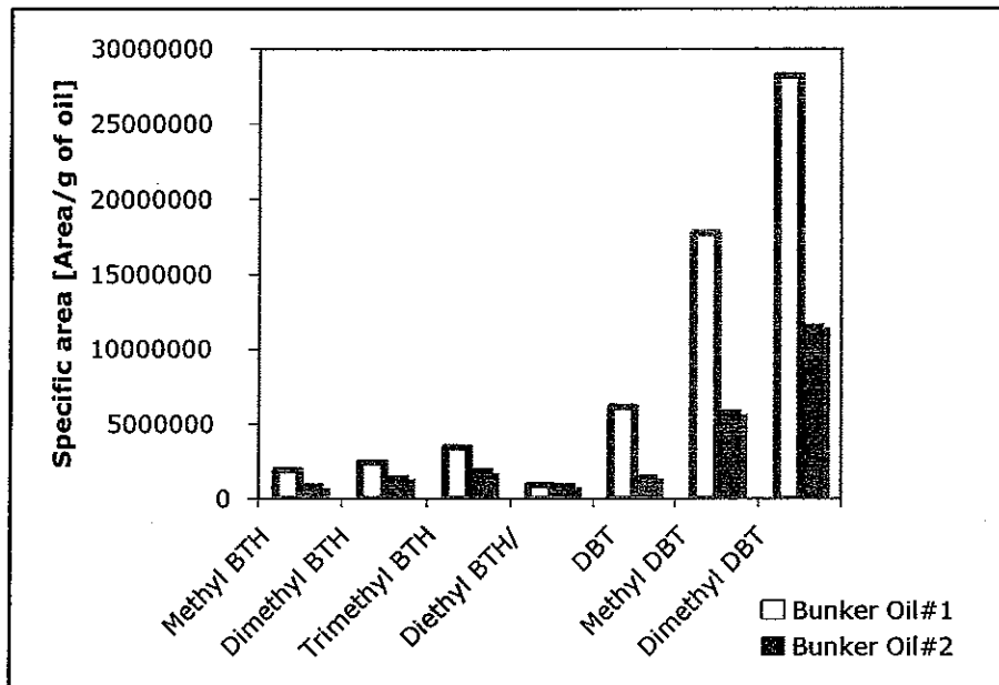
Figure 19. Comparison of intensities of organosulfur compounds in bunker oils.
