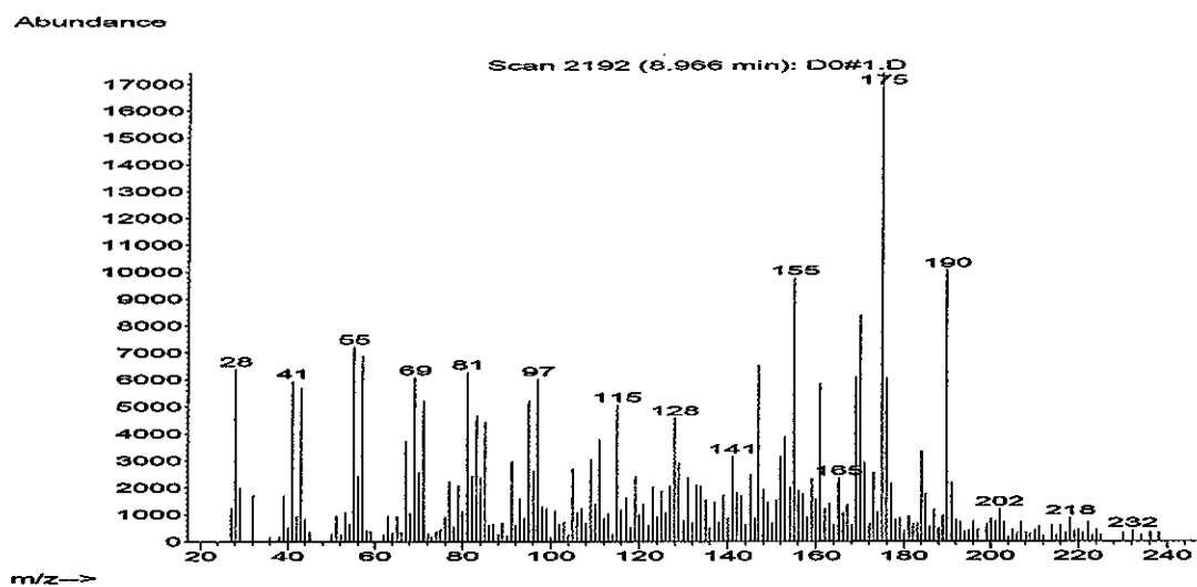
Figure 4. MS spectrum of diethyl BTH.
