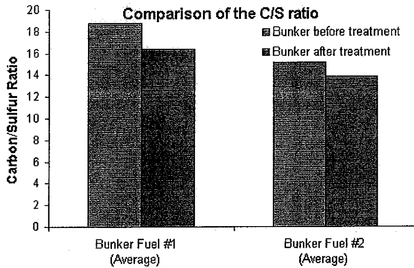
Figure 11. Comparison of the average carbon/sulfur ratio in bunker fuel #1 and #2 before and after treatment.
