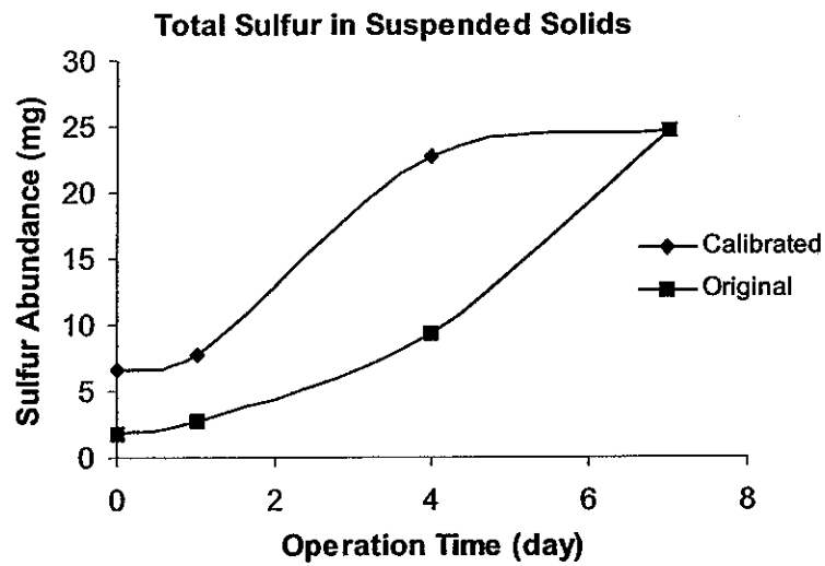
Figure 8. Total sulfur quantity in the biomass of the seed reactor.
