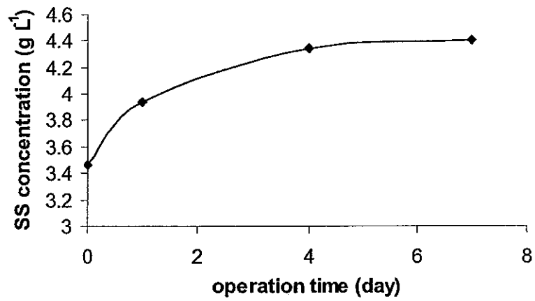
Figure 3. Change of suspended solids (SS) concentration with operation in the seed reactor.
