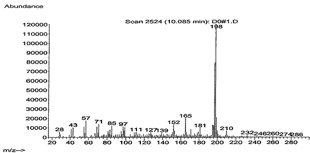
Figure 6. MS spectrum of methyl DBT.
