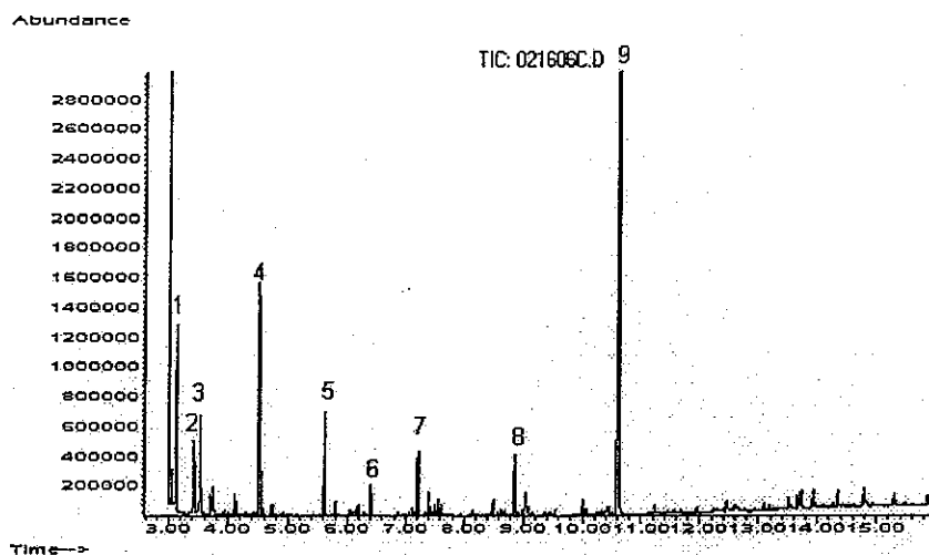
Figure 6. The GC total ion chromatogram of the n-hexane extract from the control reactor on day 6.
