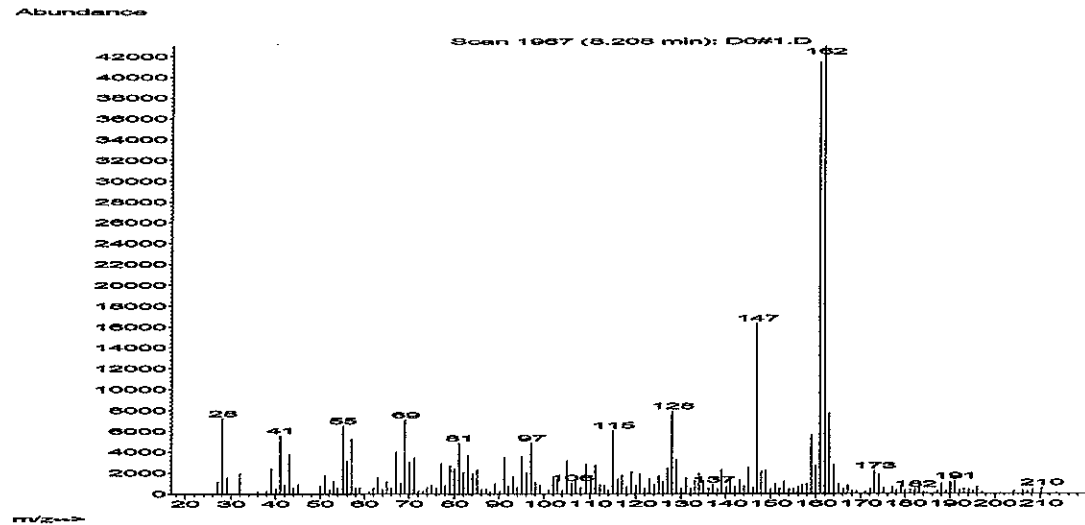
Figure 2. MS spectrum of dimethyl BTH.
