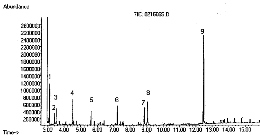
Figure 5. The GC total ion chromatogram of the n-hexane extract from the seed reactor on day 6.
