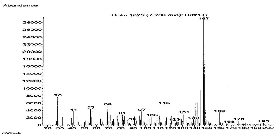
Figure 1. MS spectrum of methyl BTH.
