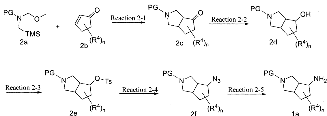
Reaction scheme 2
