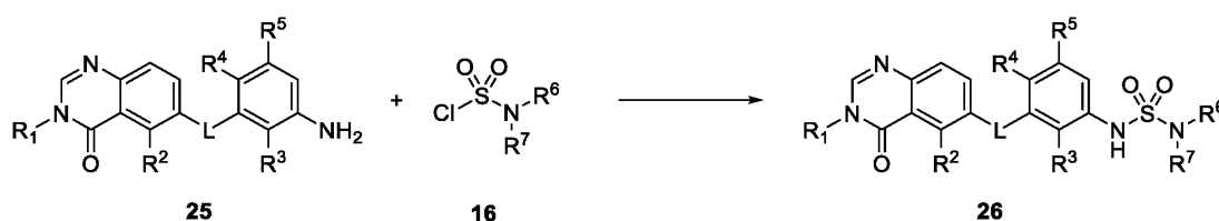
Scheme 7
