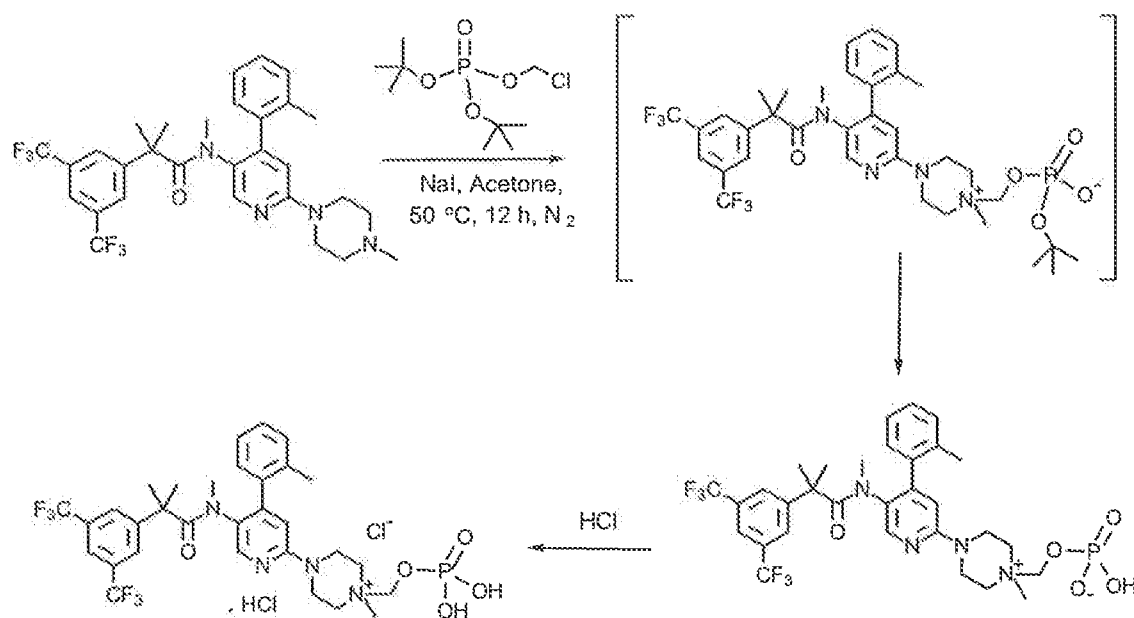
Scheme 6A
