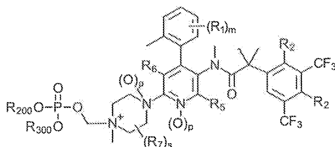
Formula (VI)
