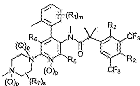
Formula (V)
