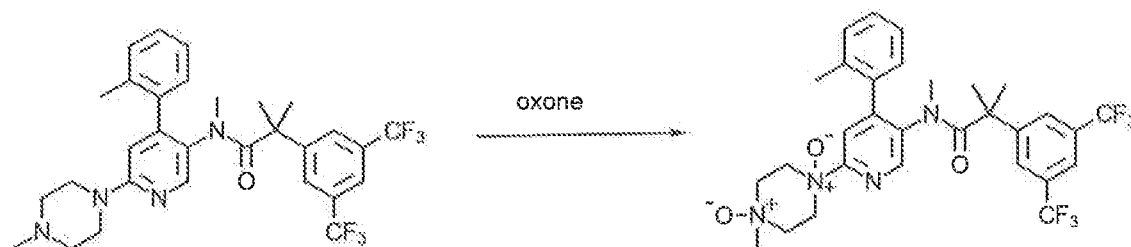
Scheme 4
