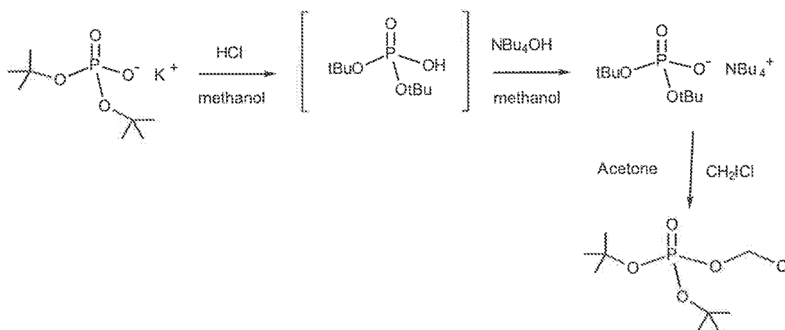
Scheme 5A
