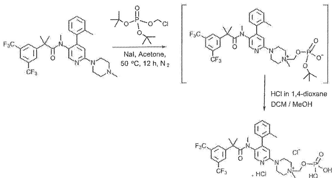
Scheme 6
