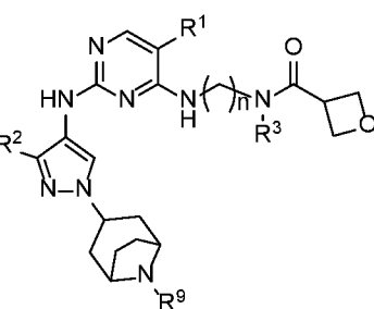
Formula IE.8
