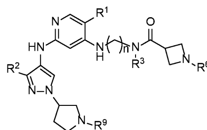
Formula IF.6
