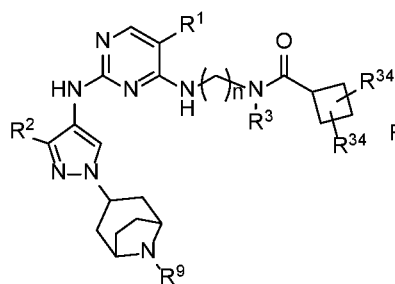
Formula IE.7
