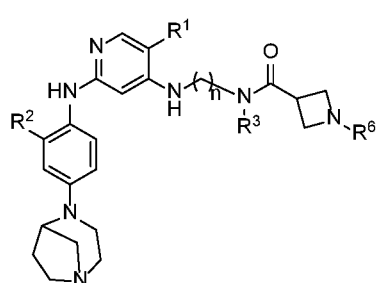
Formula IC.14
