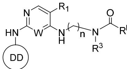
Formula ID
