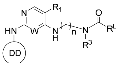
Formula ID
