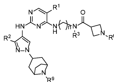
Formula IE.9
