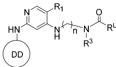
Formula IF
