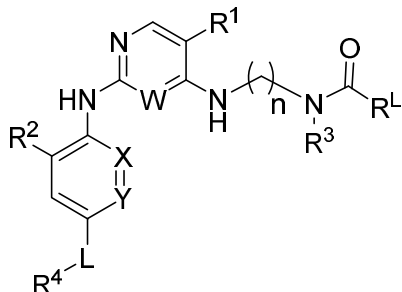
Formula IA
