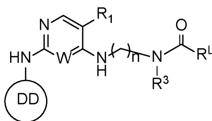
Formula ID
