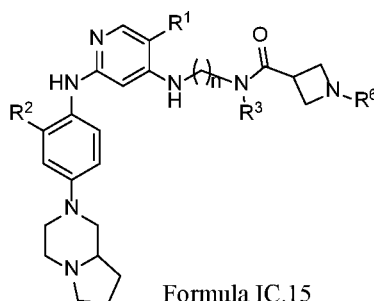
Formula IC.15
