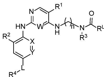
Formula 1A
