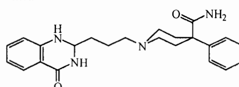
Compound 5
