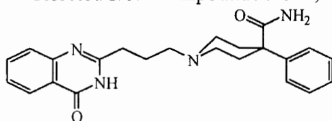
Compound 4
