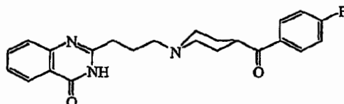
Compound 14
