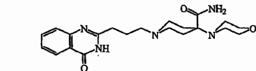
Compound 11
