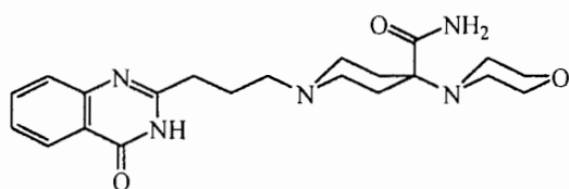
Compound 11
