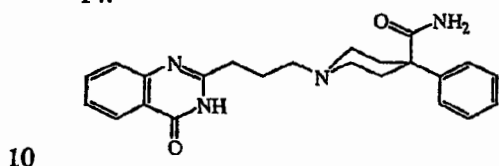
Compound 4
