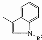
(b-8)
