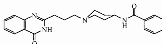
Compound 12
