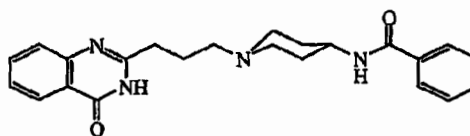
Compound 12
