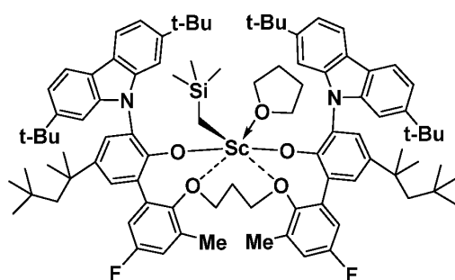
Inventive Metal-Ligand Complex 5
