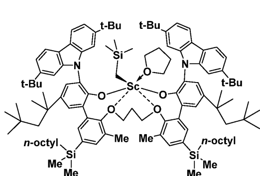
Inventive Metal-Ligand Complex 1
