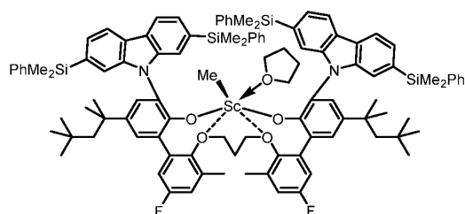
Inventive Metal-Ligand Complex 8
