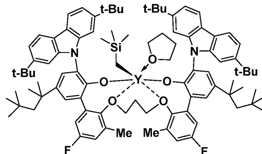
Inventive Metal-Ligand Complex 4
