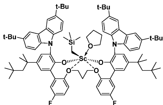
Inventive Metal-Ligand Complex 2
