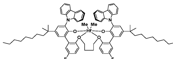
Comparative Metal-Ligand Complex 2 (C2)
