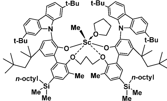
Inventive Metal-Ligand Complex 6
