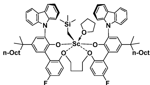
Inventive Metal-Ligand Complex 3
