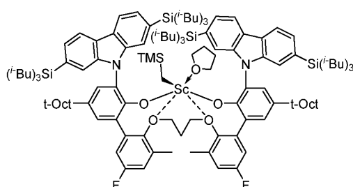
Inventive Metal-Ligand Complex 9
