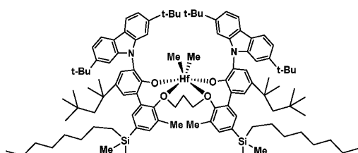
Comparative Metal-Ligand Complex 1 (C1)
