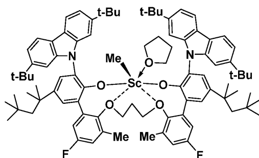
Inventive Metal-Ligand Complex 7
