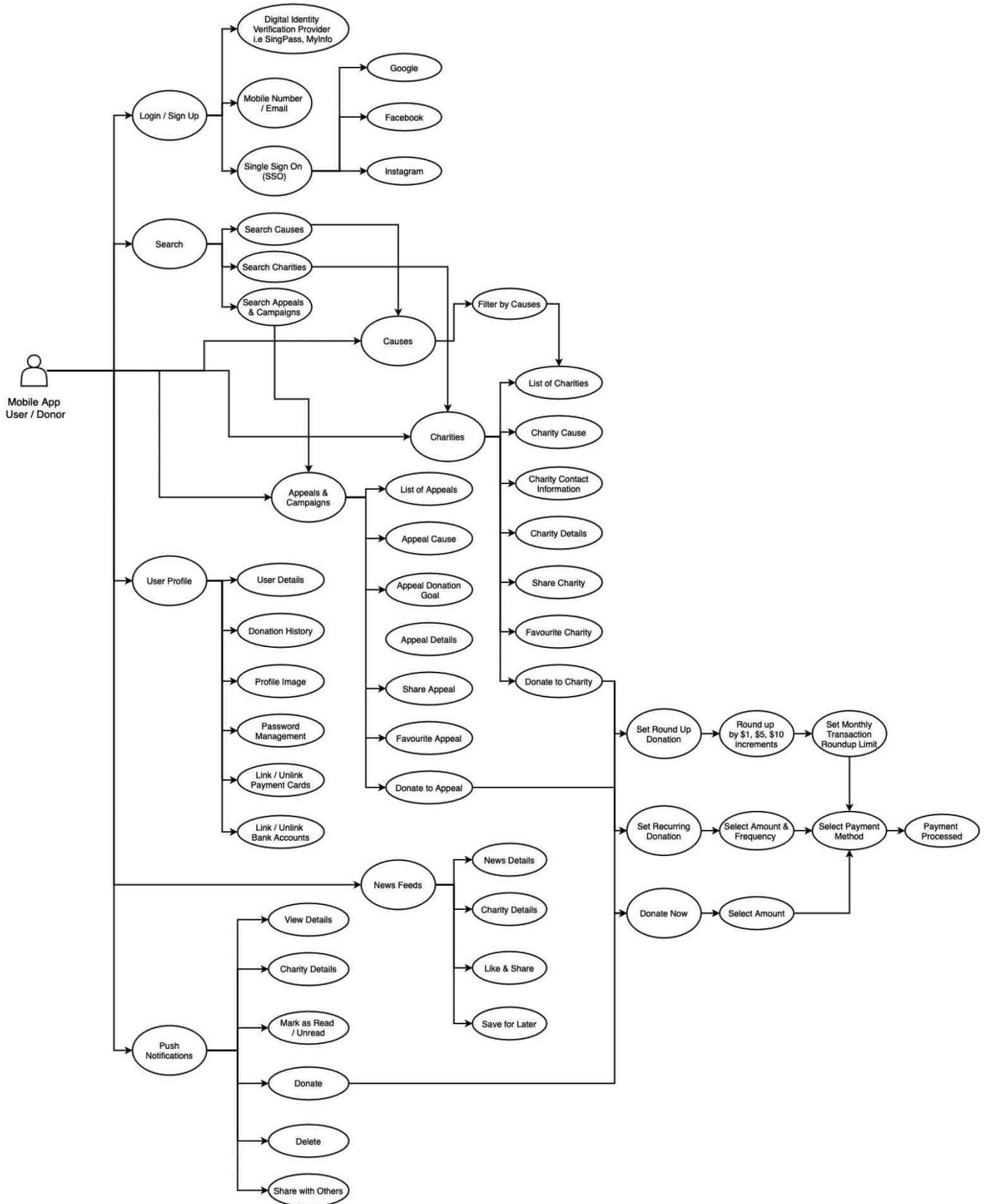
Figure 7 – Use Case of Mobile Application
