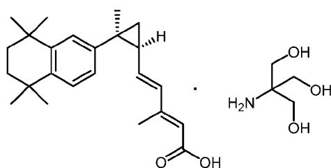
A representation of a Tris salt form of Compound 1
