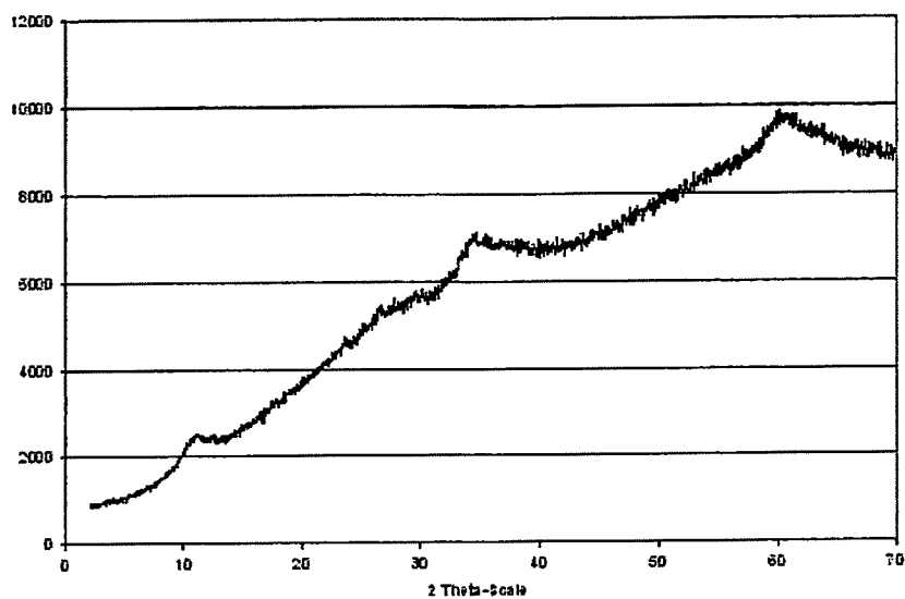
Figure 1: XRD pattern of amorphous catalyst of comparative experiment C5:
