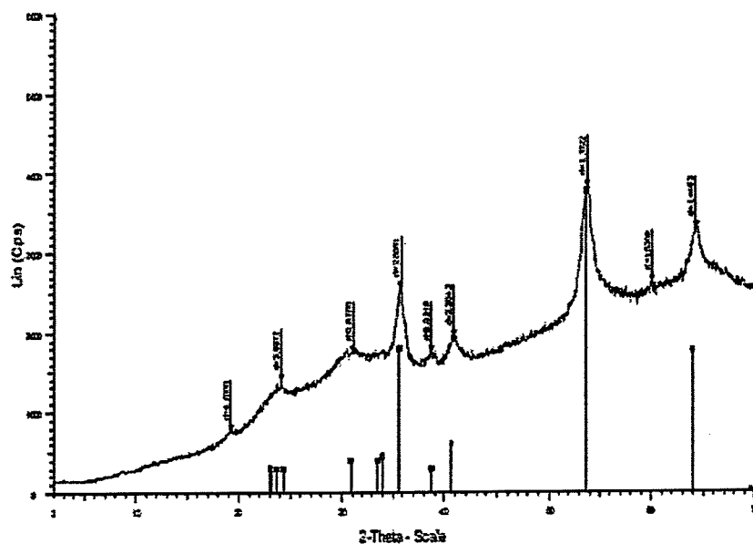
Figure 2: XRD pattern of trimetallic catalyst of comparative experiment C4
