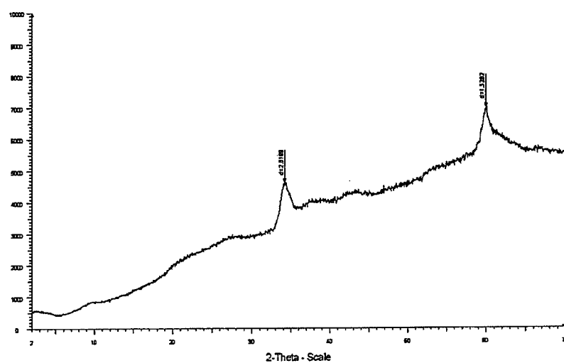
Figure 3: XRD pattern of catalyst of example E2
