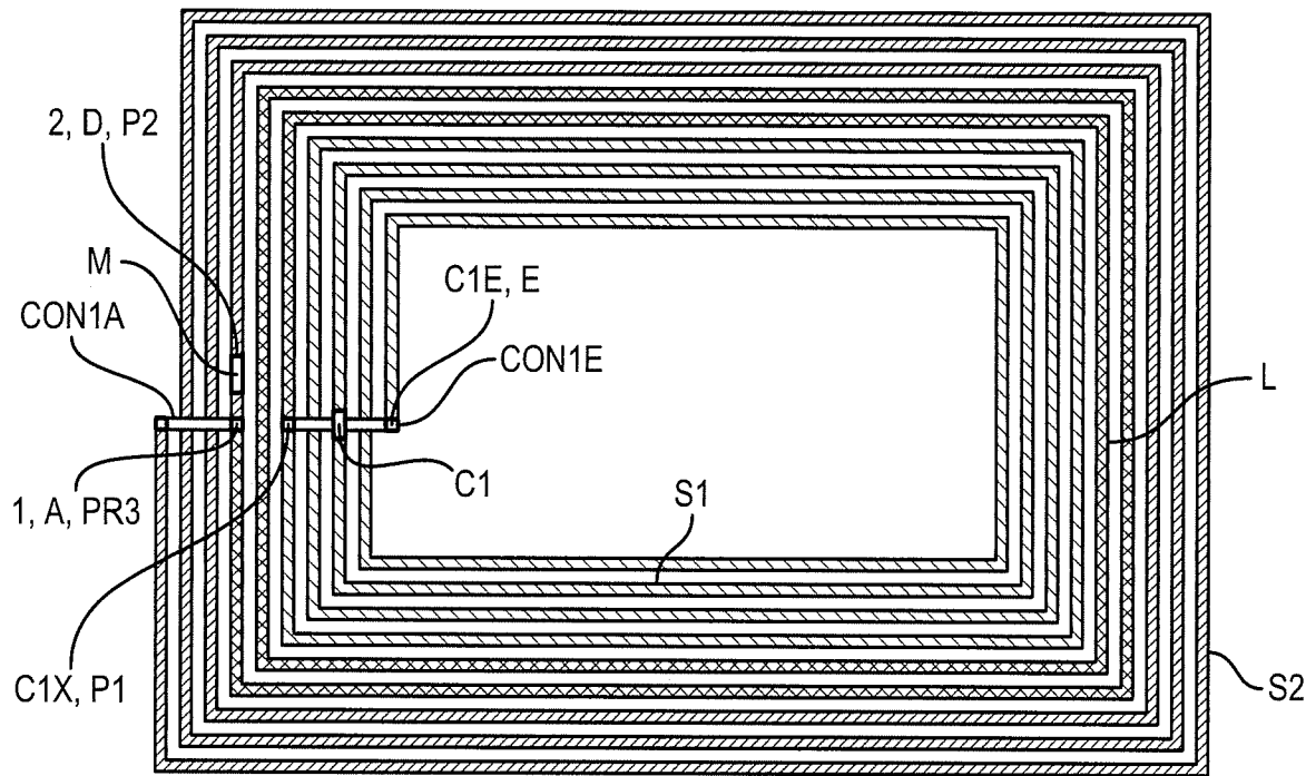
Antenna - 21BB
