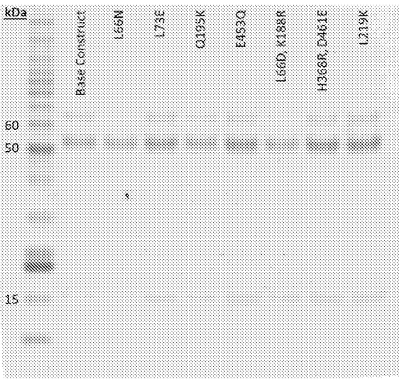
Electrostatic mutations
