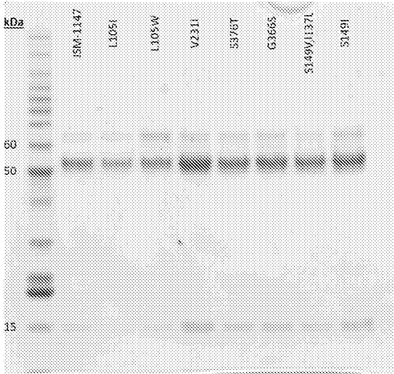
Cavity mutations
