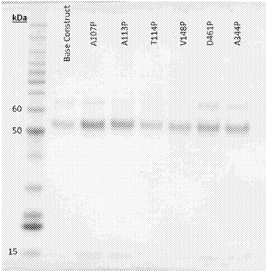
Proline mutations
