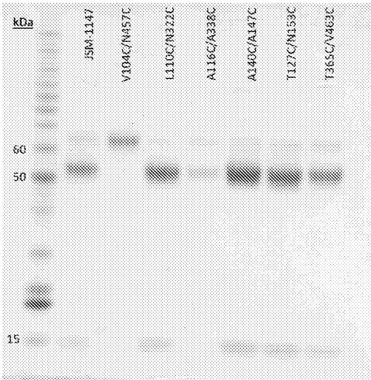
Disulfide mutations
