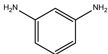
m-phenylenediamine
