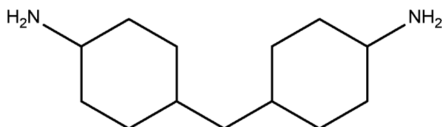
4,4'-methylenebis(cyclohexylamine)
