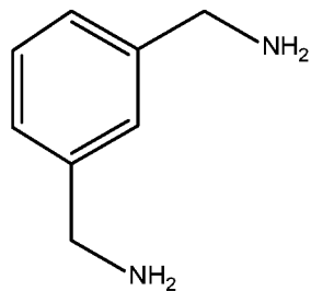
m-Xylylenediamine
