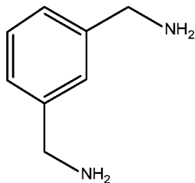
m-xylylenediamine
