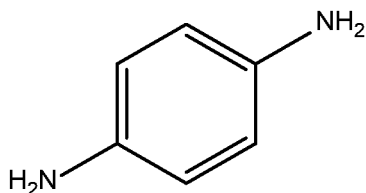
p-phenylenediamine
