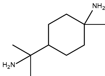
1,8-p-menthane-1,8-diamine
