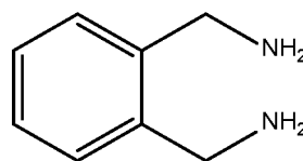
o-Xylylenediamine
