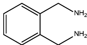
o-Xylylenediamine
