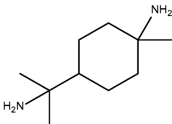
1,8-p-menthane-1,8-diamine
