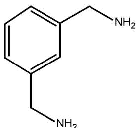
m-xylylenediamine
