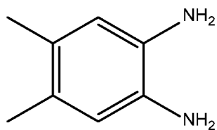
4,5-dimethyl-1,2-phenylenediamine
