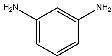
m-phenylenediamine
