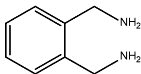
o-xylylenediamine
