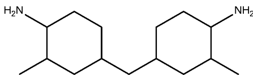
4,4'-methylenebis(2-methylcyclohexylamine)
