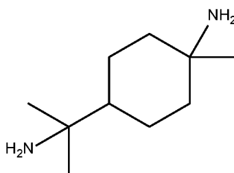
1,8-p-Menthanediamine
