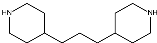
4,4'-trimethylenedipiperidine
