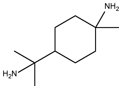
1,8-p-menthane-1,8-diamine
