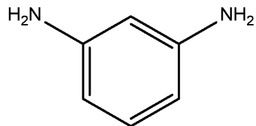
m-phenylenediamine
