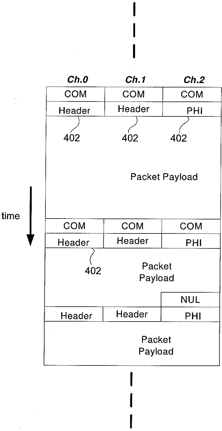
Main Link Packet Format
