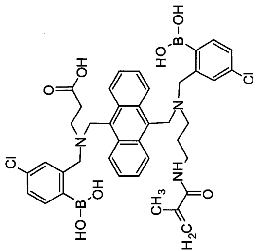
4-Chloro (32b)
