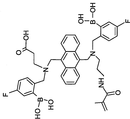
5-Fluoro (32a)
