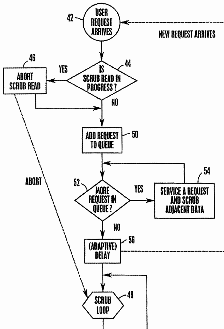
Fig. 4 Interrupt of Scrub with Delay, opportunistic options
