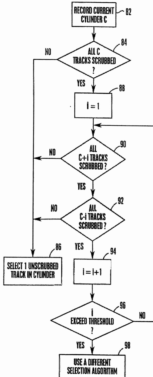
Fig. 6 Scrub Nearest Data Unit
