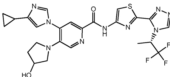
4-(4-cyclopropyl-1H-imidazol-1-yl)-5-(3-hydroxypyrrolidin-1-yl)-N-(2-(4-((S)-1,1,1-trifluoropropan-2-yl)-4H-1,2,4-triazol-3-yl)thiazol-4-yl)picolinamide;
