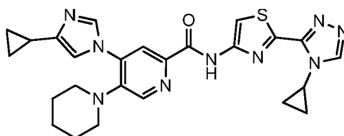
4-(4-cyclopropylimidazol-1-yl)-N-[2-(4-cyclopropyl-1,2,4-triazol-3-yl)-1,3-thiazol-4-yl]-5-piperidin-1-ylpyridine-2-carboxamide;
