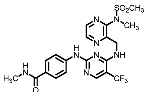
Formula (I-d)
