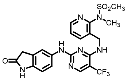
Formula (I-e)
