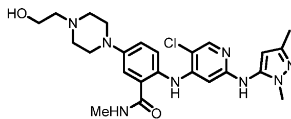
Formula (I-c4)
