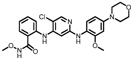
Formula (I-c1)
