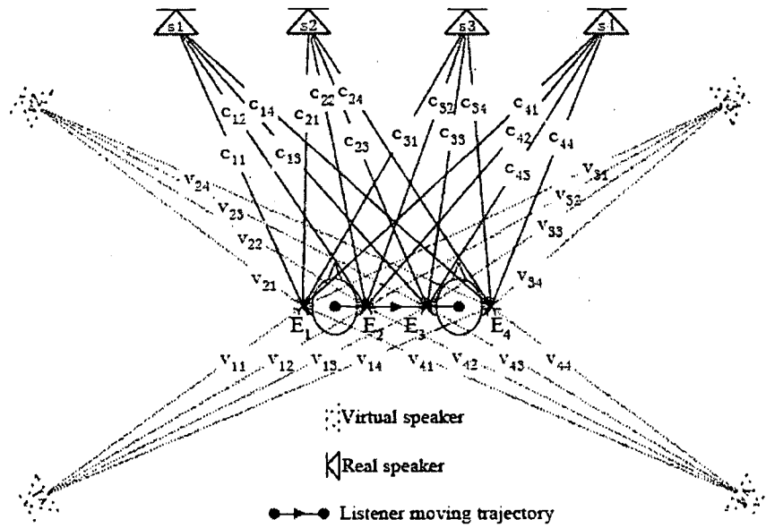
Fig3. Surround audio reconstruction with loudspeaker array (4 speakers)
