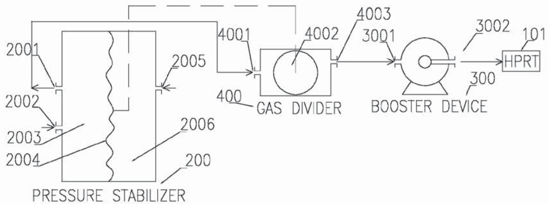
(FIGURE 1) TWO TYPE PPSS CONNECTION
