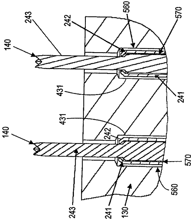
Fig. 5 Prior Art
