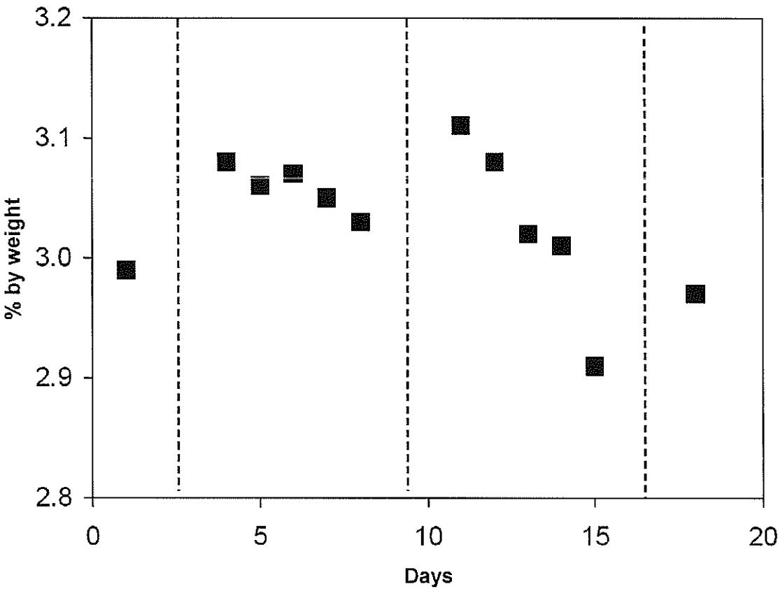
Methyldi-n-hexylamine concentration in stream (8)
