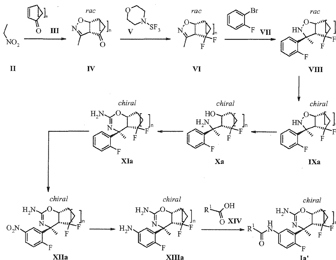
Scheme 1: Synthesis of compounds of formula Ia'
