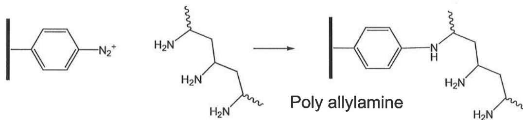
Amino acids
