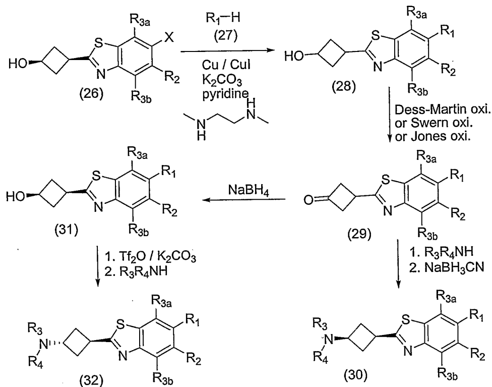
Scheme 6
