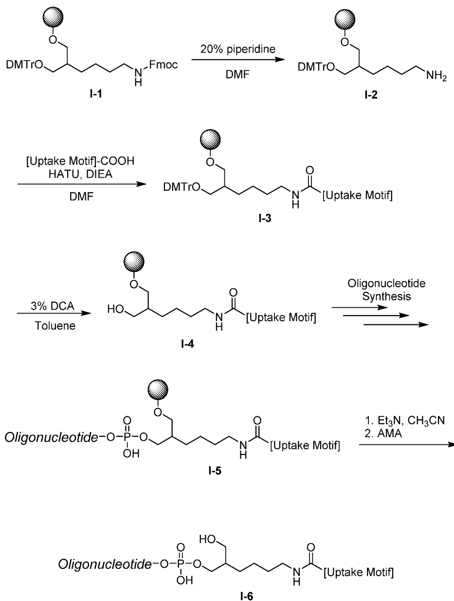
Scheme I: Conjugation of an Uptake Motif to the 3' end of an oligonucleotide
