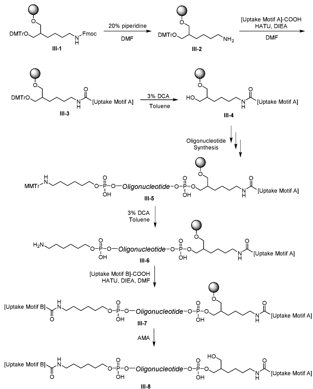
Scheme III: Double Conjugation of Uptake Motifs at both ends of an oligonucleotide
