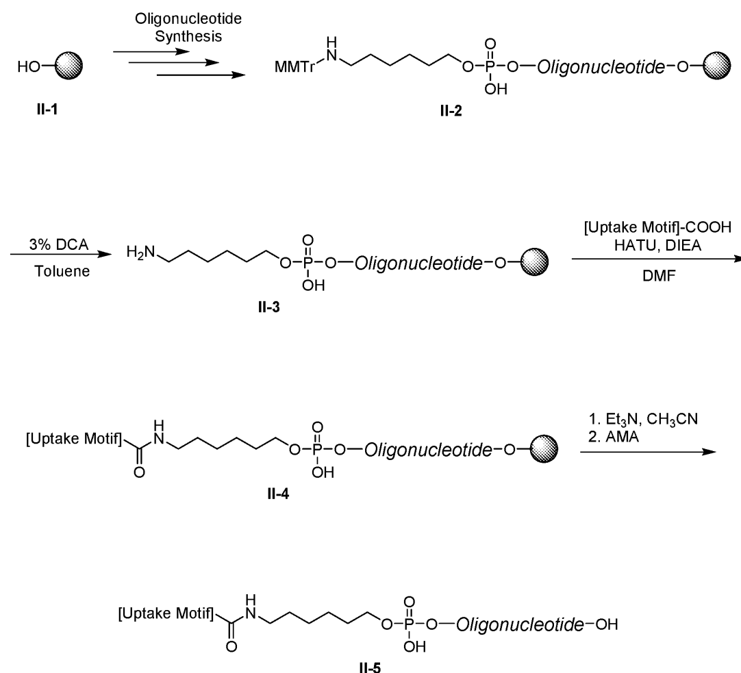
Scheme II: Conjugation of an Uptake Motif to the 3' end of an oligonucleotide
