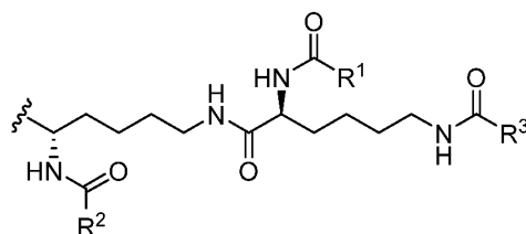
Structure of uptake motif DTx-04
