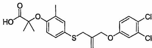
Compound 4
