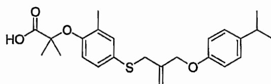
Compound 6
