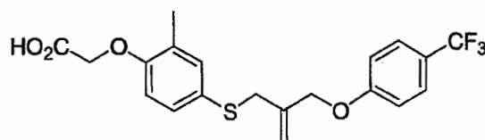
{2-Methyl-4-[2-(4-trifluoromethyl-phenoxy)-allylsulfanyl]-phenoxy}-acetic acid
