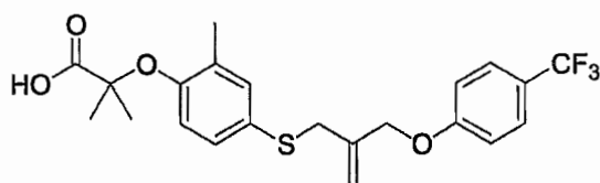
Compound 1
