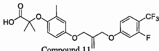
Compound 11
