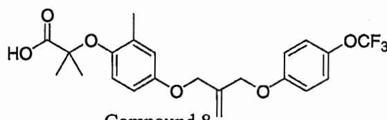
Compound 8
