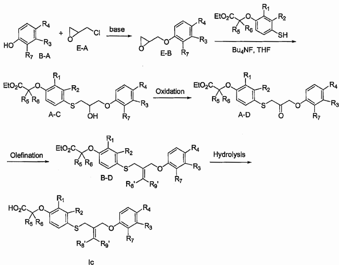
Scheme E
