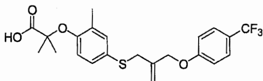
Compound 1
