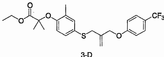
2-Methyl-2-{2-methyl-4-[2-(4-trifluoromethyl-phenoxy)methyl]-allylsulfanyl]-phenoxy}-propionic acid ethyl ester
