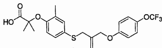
Compound 2
