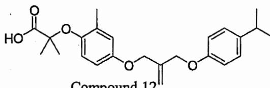
Compound 12
