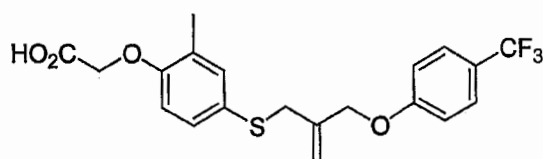
{2-Methyl-4-[2-(4-trifluoromethyl-phenoxy)-allylsulfanyl]-phenoxy}-acetic acid
