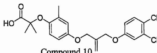
Compound 10
