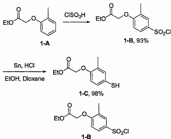
(4-Chlorosulfonyl-2-methyl-phenoxy)-acetic acid ethyl ester
