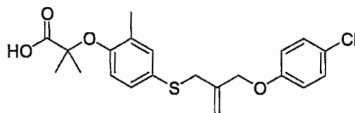
Compound 3
