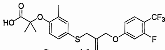
Compound 5
