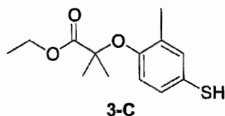
2-(4-Mercapto-2-methyl-phenoxy)-2-methyl-propionic acid ethyl ester
