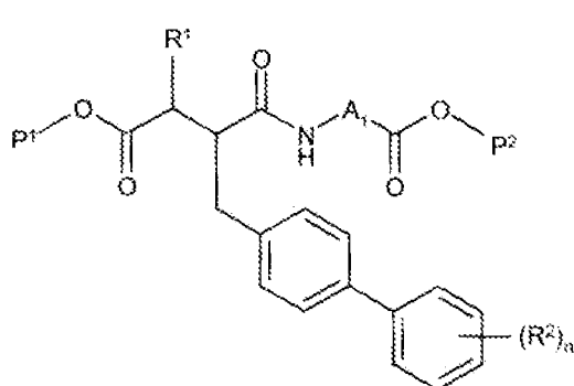
Intermediate D
