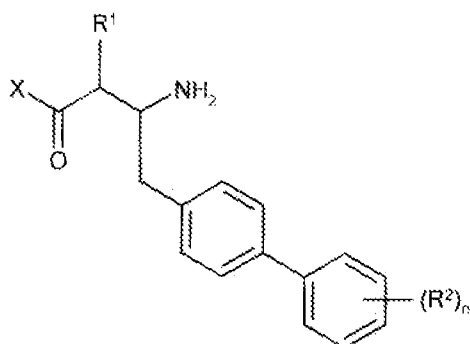
Intermediate H
