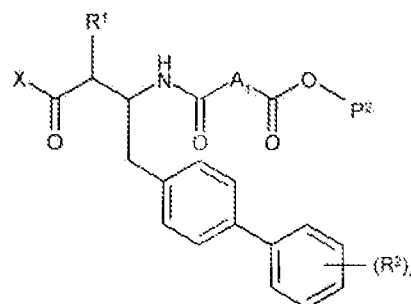
Intermediate B
