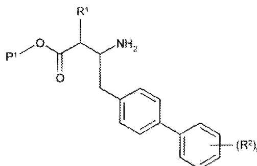
Intermediate I
