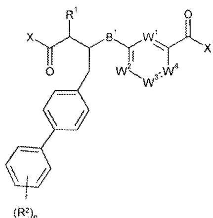
Formula VI
