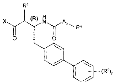
Formula VIIA
