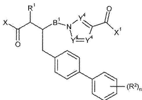
Formula V
