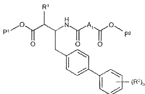
Intermediate A
