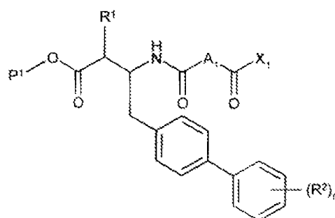
Intermediate C
