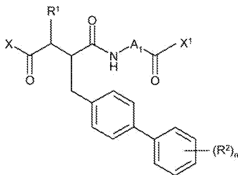
Formula III
