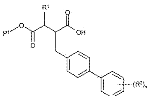
Intermediate M
