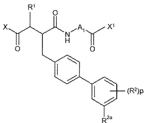
Formula IIIB
