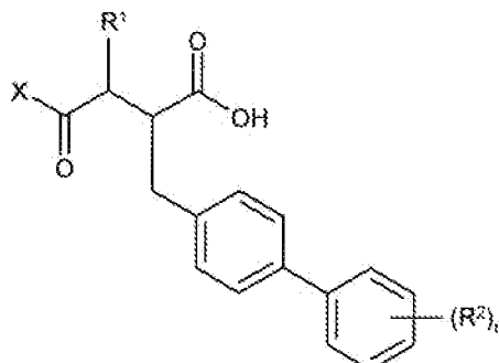
Intermediate N
