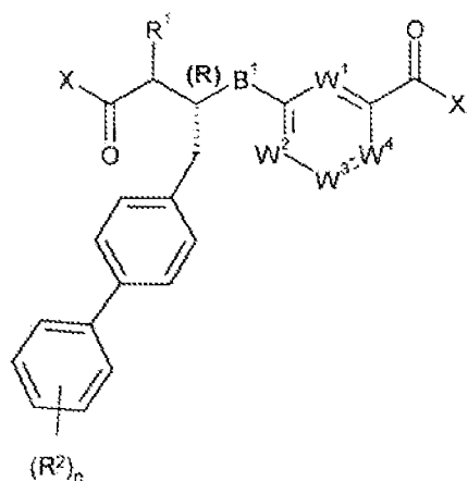
Formula VIA
