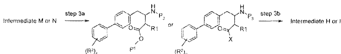
Scheme 3
