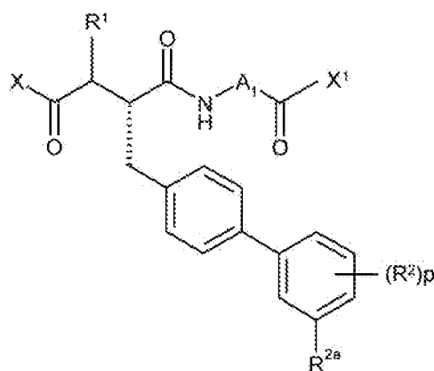
Formula IIIC
