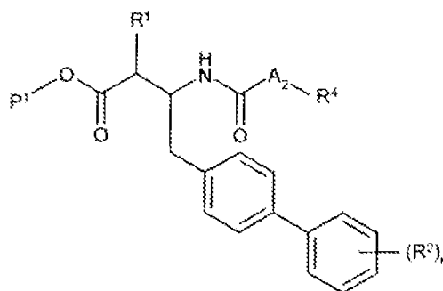
Intermediate G
