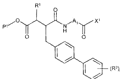
Intermediate F
