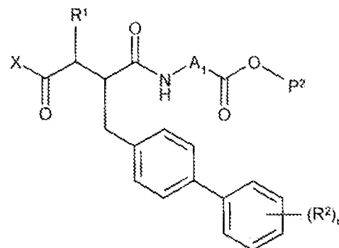
Intermediate E
