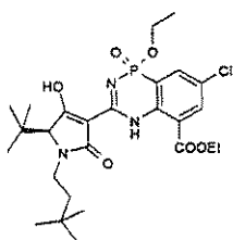
(S)-isomer of (IV-142)
