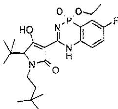
(S)-isomer of (IV-85)
