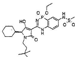
(S) isomer of (IV-119)
