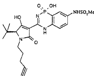
(S)-isomer of (IV-135)
