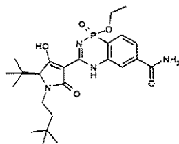
(S)-isomer of (IV-160)
