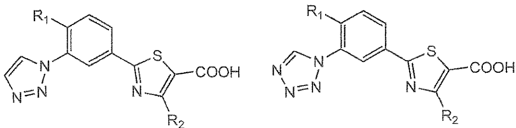
[Chemical Formula 6]
