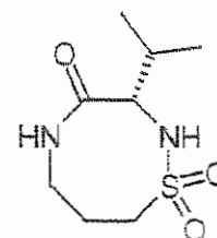
Compound D8
