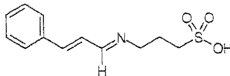
Compound M5
