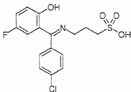
Compound M7
