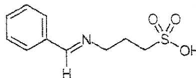
Compound M4
