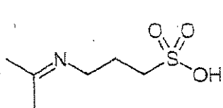
Compound M1
