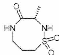
Compound D7
