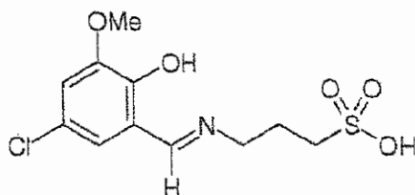
Compound M9
