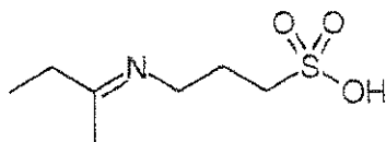
Compound M3
