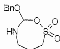
Compound D4
