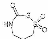
Compound D6
