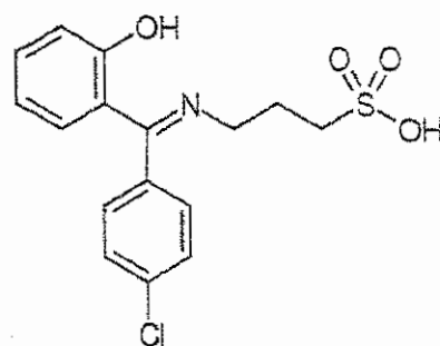
Compound M8
