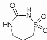
Compound D5
