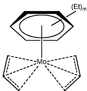
Formula II(a)
