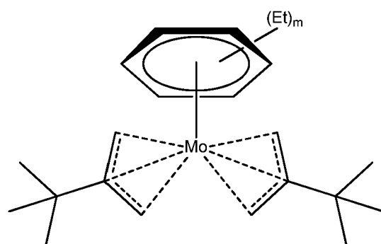
Formula II(b)
