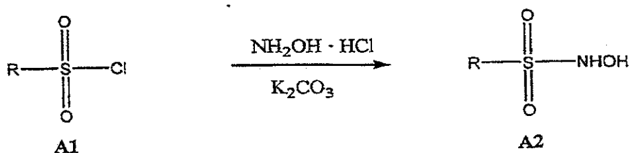
Scheme A. General Synthesis of N -Hydroxysulfonamides.
