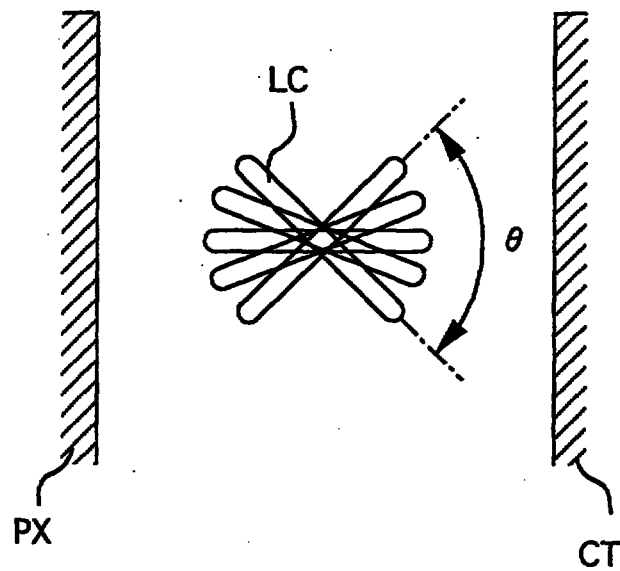
(a) State of voltage OFF (High penetration rate)
