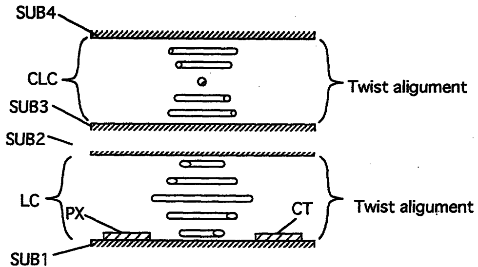
(a) State of voltage OFF (High penetration rete)
