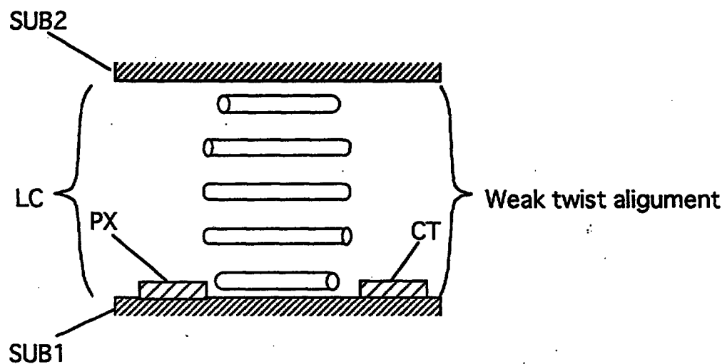
(a) State of voltage OFF (Low Penetration rate)
