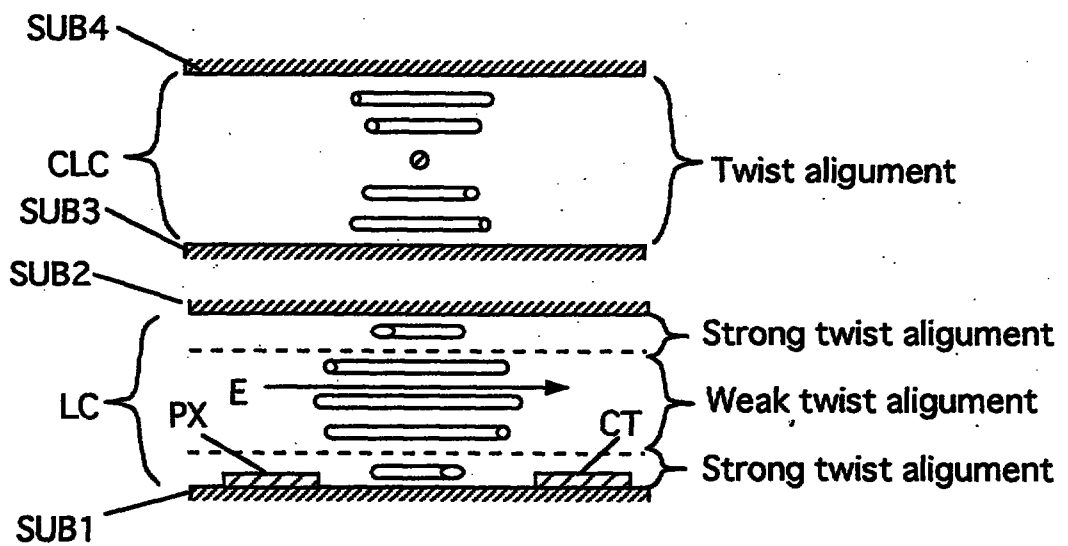
(b) State of voltage ON (Low penetration rete)
