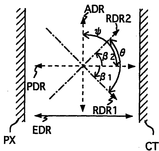
(a) Liquid Crystal cell for drive
