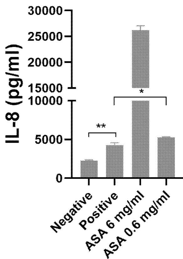
FIG. 4B IL-8 measurement corresponding to 2A, 2B
